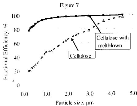
Figure 7. Cellulose and cellulose-meltblown media performance
