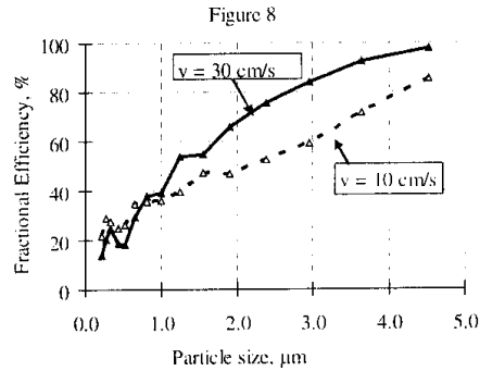
Figure 8. Synthetic filter and its fractional efficiency
