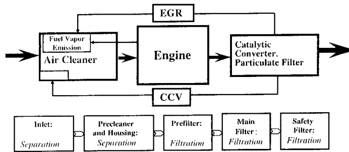
Figure 1. Total engine air and exhaust systems
