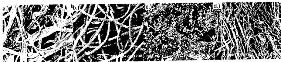
Figure 5. a) Structure of cellulose, b) synthetic, c) nanofiber filter media with captured dust particles, and d) new type prefilter
