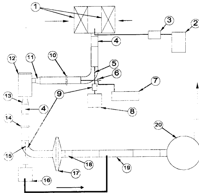
Figure 10. SAE/ISO Fractional efficiency test stand configuration
