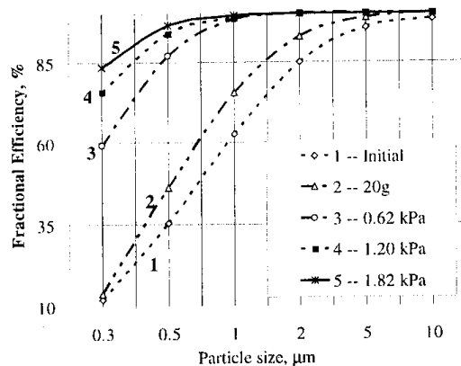
Figure 9. Fractional efficiency of a panel air cleaner with cellulose air filter element.
