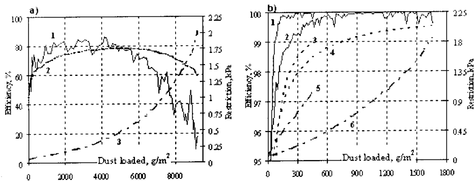
Figure 11. Continuous gravimetric efficiency: a) - high porosity synthetic nonwoven prefilter (1- incremental efficiency, 2 - cumulative efficiency, 3 - pressure drop), b) - multilayer synthetic car air filter media (1- incremental efficiency for AC Fine dust, 2 - incremental efficiency for AC Coarse dust, 3- cumulative efficiency for AC Fine dust, 4 - cumulative efficiency for AC Coarse dust, 5- pressure drop for media loaded with AC Fine dust, 6 - pressure drop for media loaded with AC Coarse dust).
