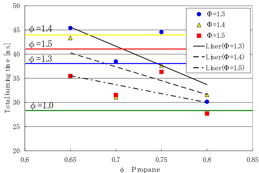
Fig.4 Total burning time vs. equivalence ratio
