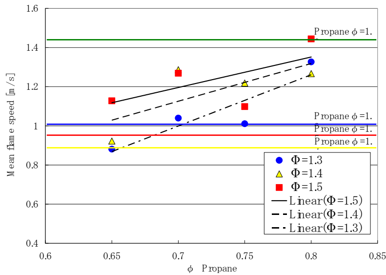
Fig.5 Mean flame speed
