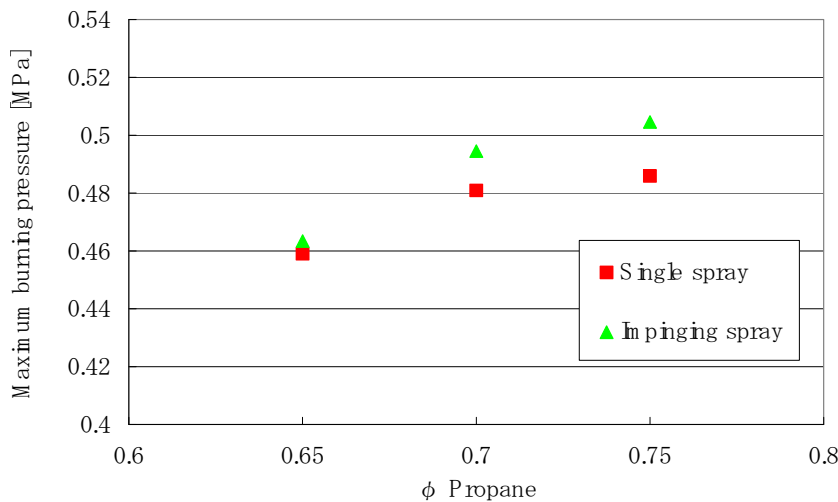
Fig.2 Maximum burning pressure vs. equivalence ratio
