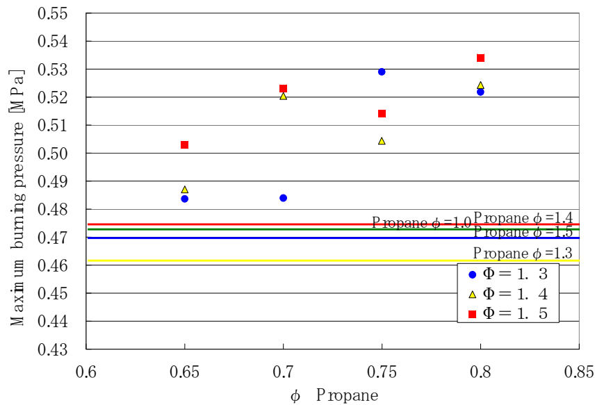
Fig.3 Maximum burning pressure vs. equivalence ratio
