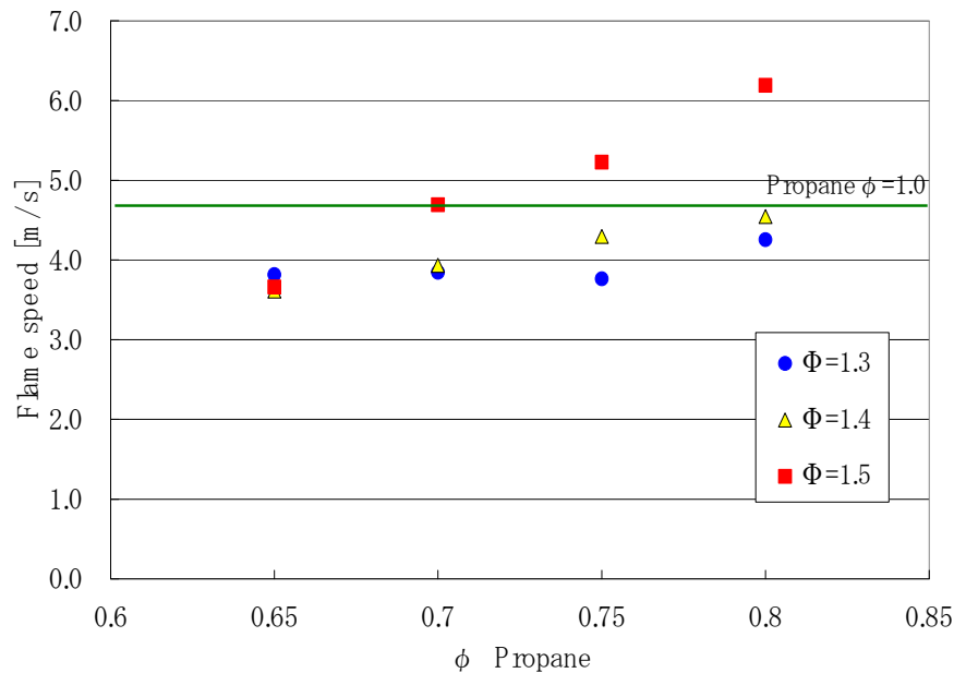
Fig.6 Flame speed
