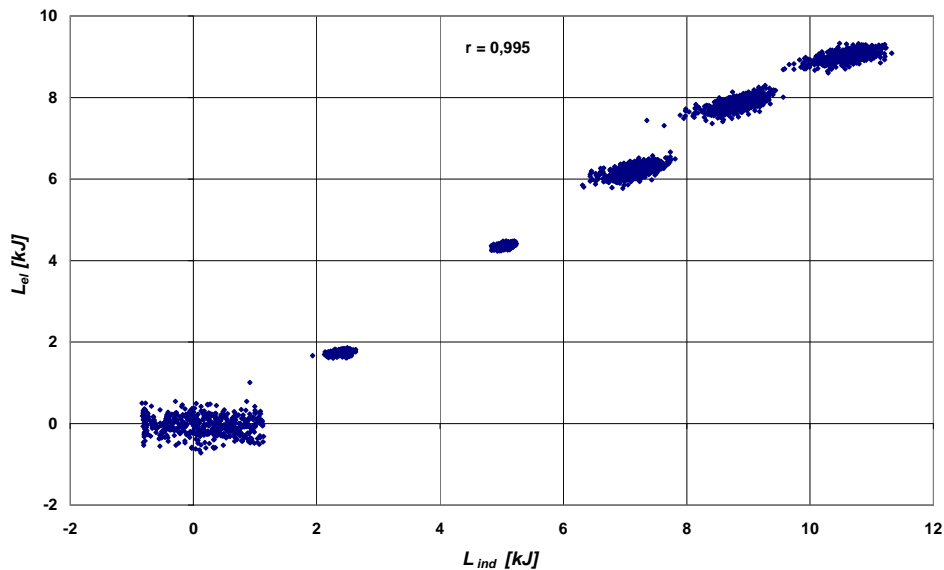
Fig.3. Correlation between indicated work calculated in interval at 360^\circ to 450^\circ\text{CA} and electric energy generated in interval at 602^\circ to 692^\circ\text{CA}
