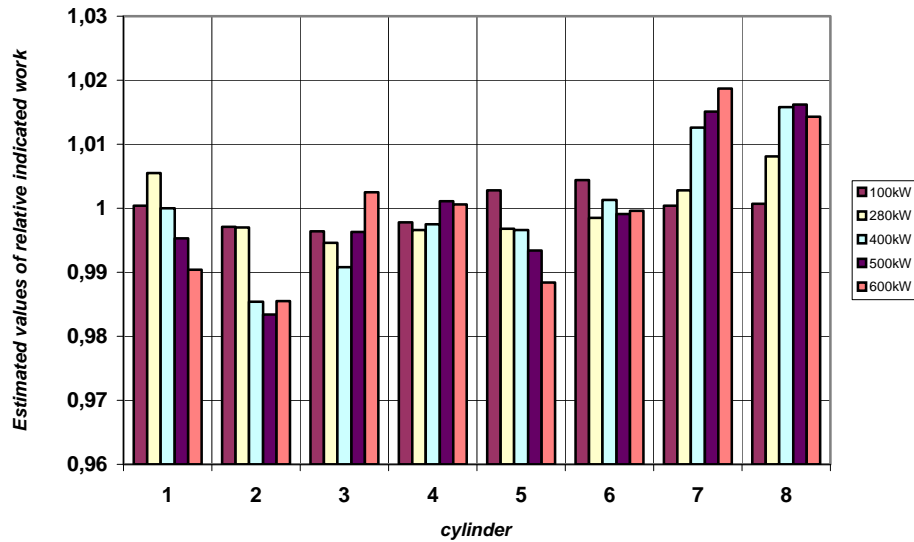
Fig.6. Estimated values of relative indicated work obtained on the basis of electric current value
